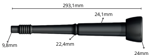
4075 - Insuflador Ultraliner DL 016U - 10 adapt. fockink
