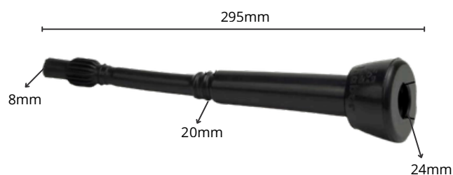
7615 - Teteira borracha inabor adapt. 2 aneis enc. 8mm REF 4169
